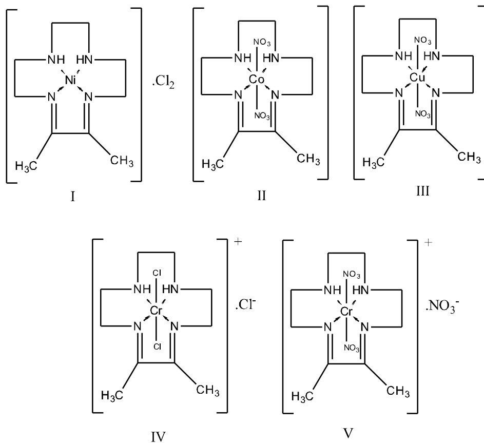
Fig. 1 Proposed Structures of the synthesized complexes of [\text{Me}_2(12)\text{dieneN}_4]
